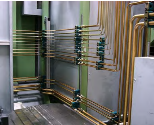
Fig. 10 Proper attachment of pipelines with pipe supports
