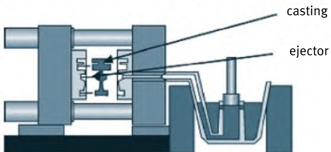
Figure 22 Schematic representation of the course of the die casting process: (a) hot chamber die casting machine, (b) cold chamber die casting machine
