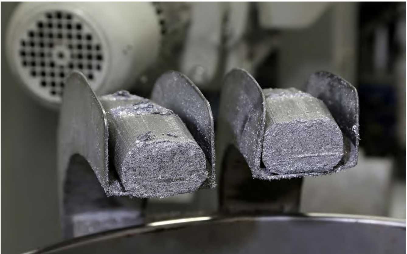
Figure 36 Briquetting system
