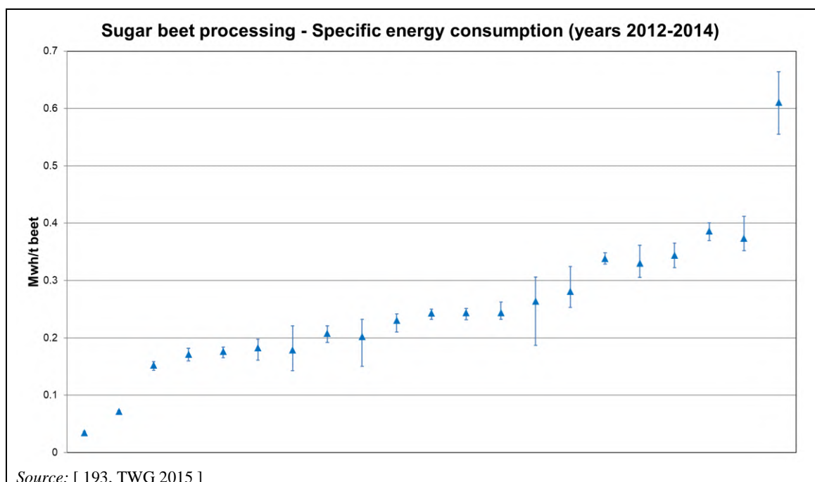
Figure 15.3: Specific energy consumption (MWh/tonne of sugar beet) from sugar beet processing
