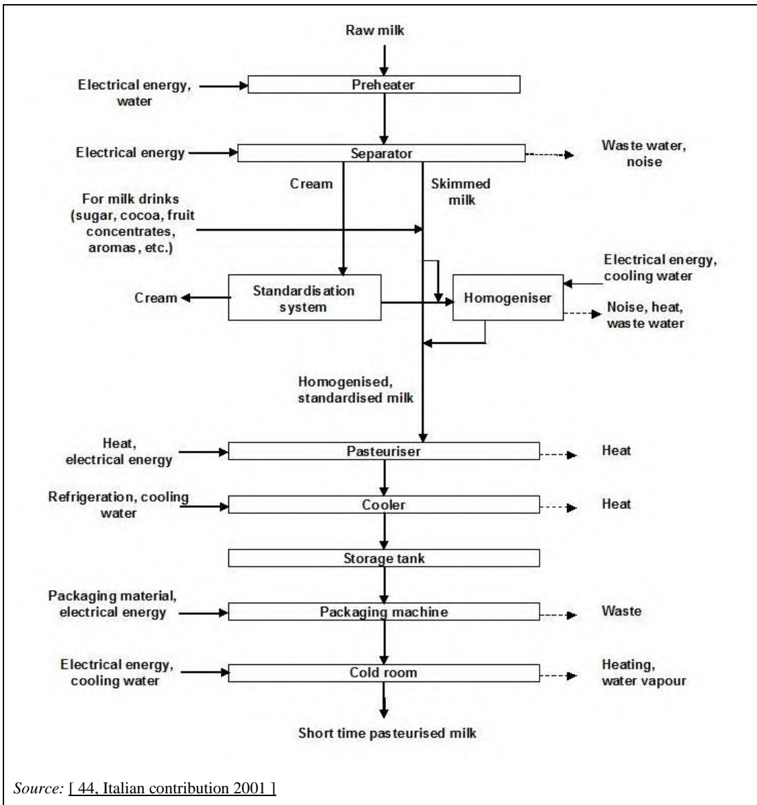
Figure 5.4: Short-time pasteurised milk process
