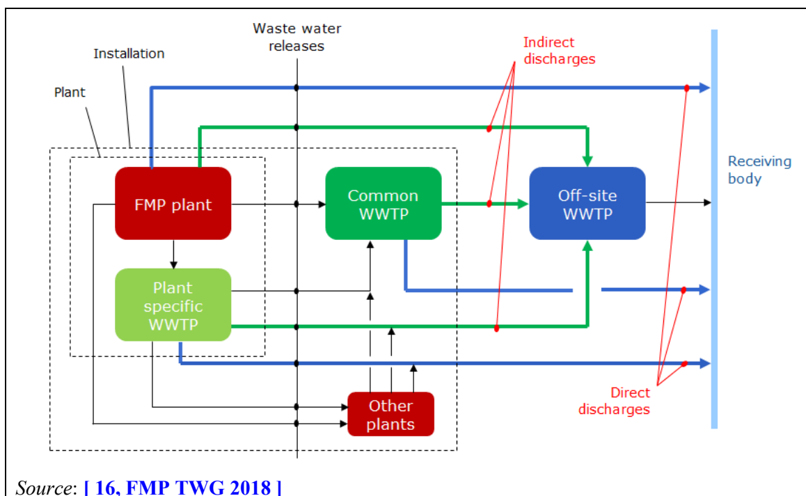
Figure 11.1: Schematic of a generic waste water system
