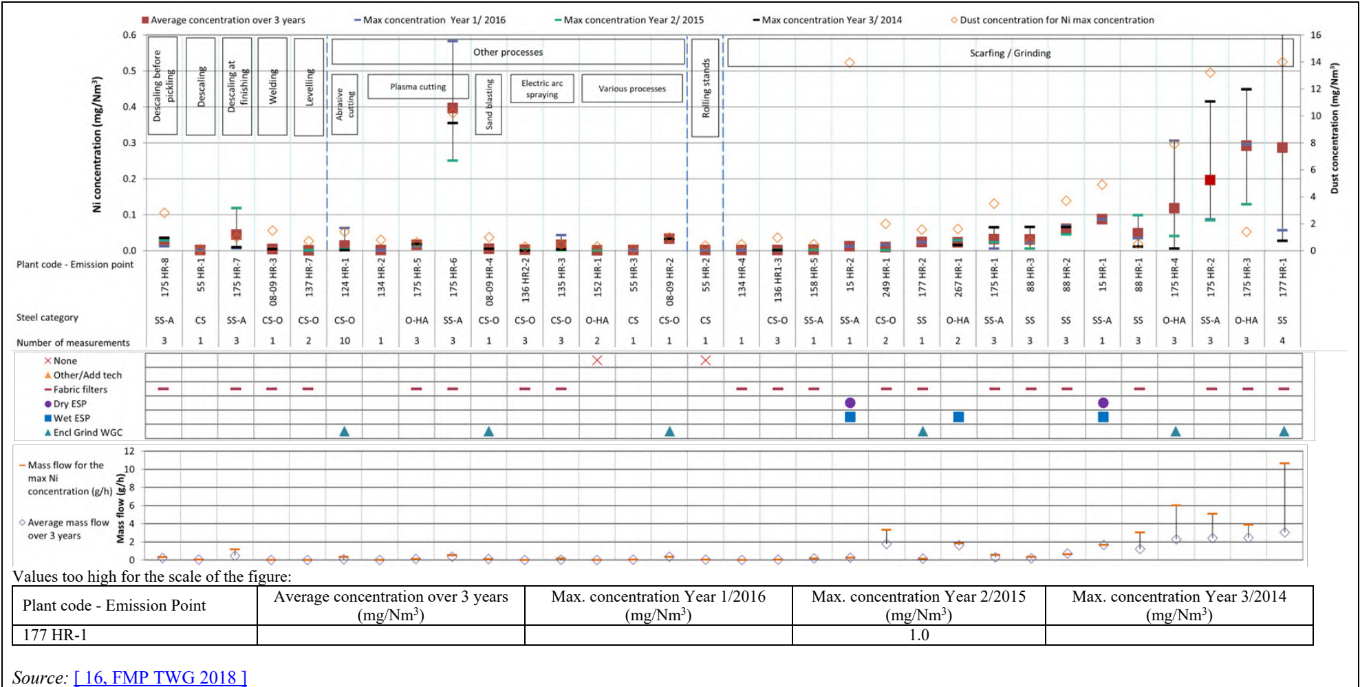
Figure 2.50: Nickel emissions from mechanical processing, scarfing and welding (in mg/Nm 3 )
