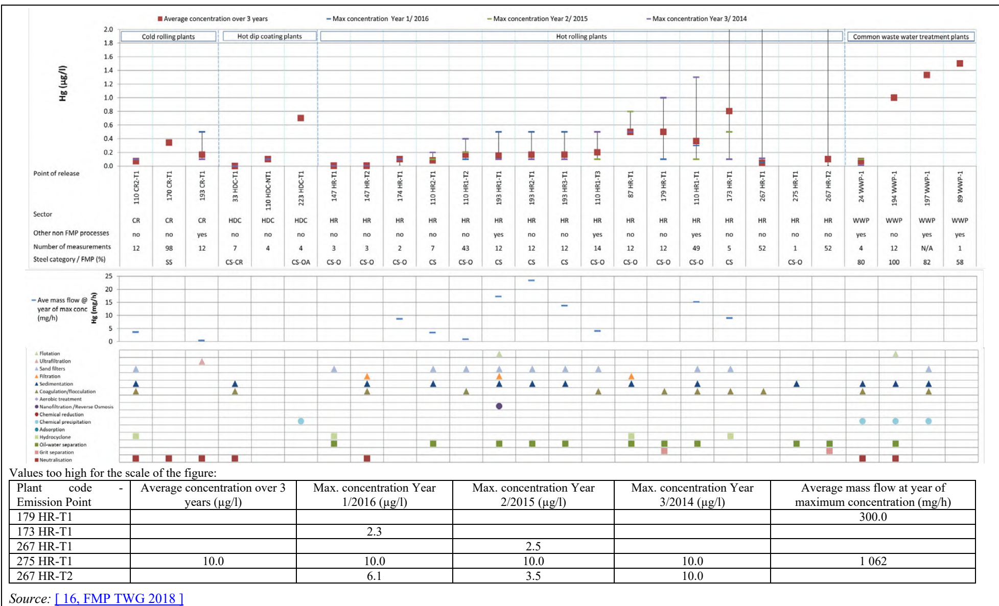
Figure 7.20: Mercury emissions (in µg/l) for direct discharges
