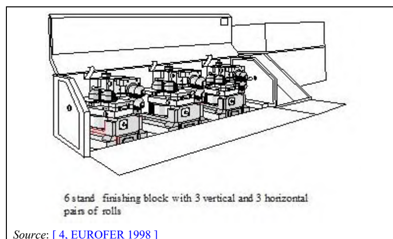
Figure 2.22: Roller arrangement of wire rod finishing section
