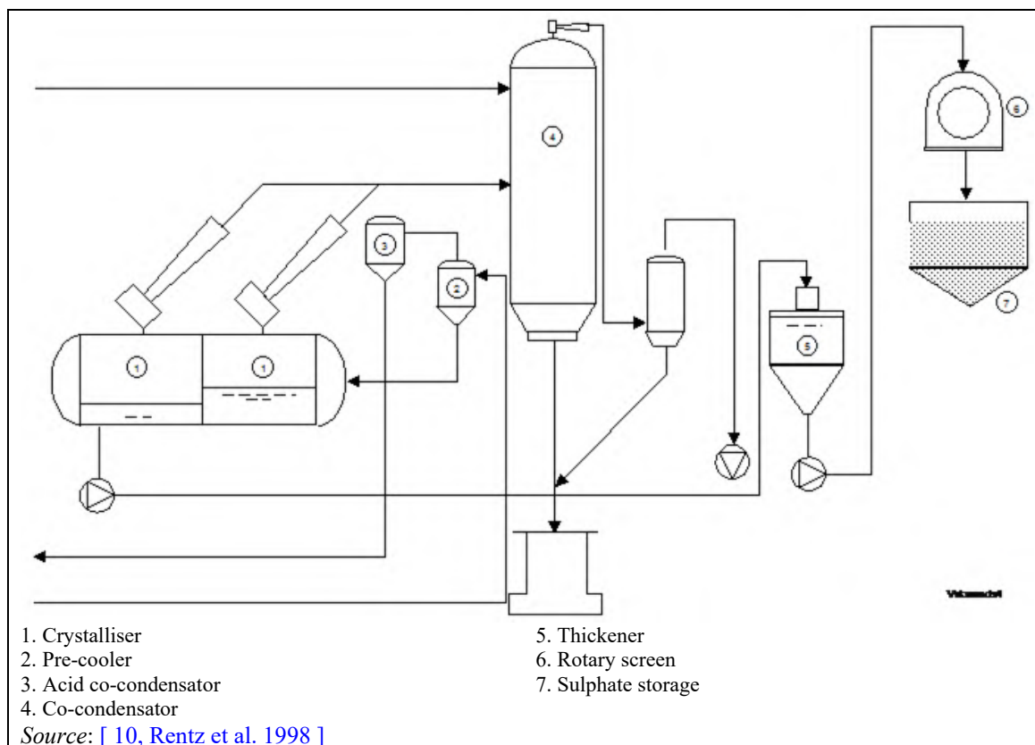
Figure 8.25: Vacuum cooling crystallisation process for \text{H}_2\text{SO}_4
