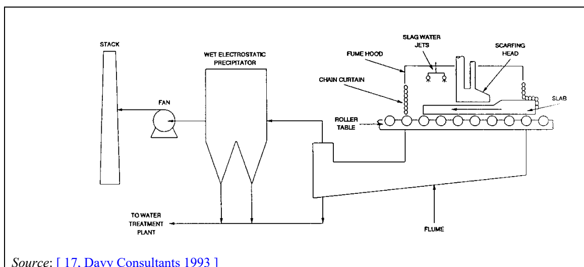
Source: [ 17, Davy Consultants 1993 ] Figure 2.73: Scarfing abatement flowsheet (example with wet EP)
