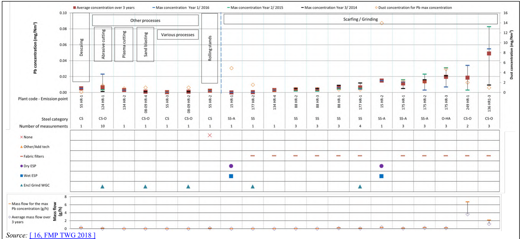
Figure 2.49: Lead emissions from mechanical processing, scarfing and welding (in mg/Nm³)
