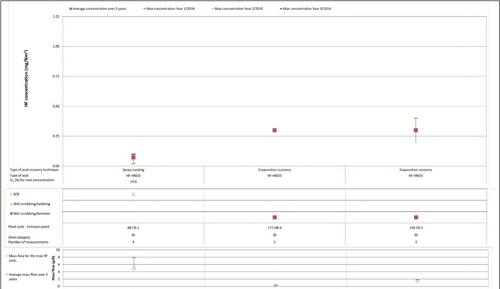
Figure 7.5: HF emissions from acid recovery (in mg/Nm 3 )
