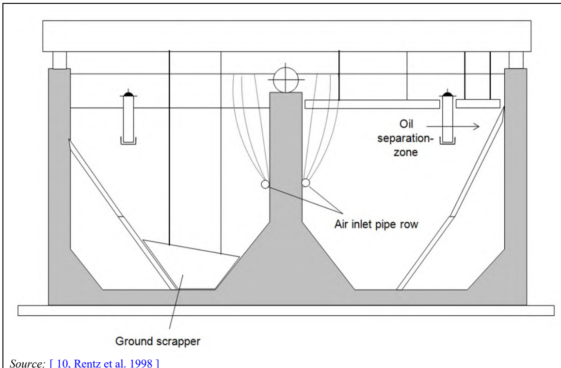
Figure 2.108: Aerated fine scale-trap
