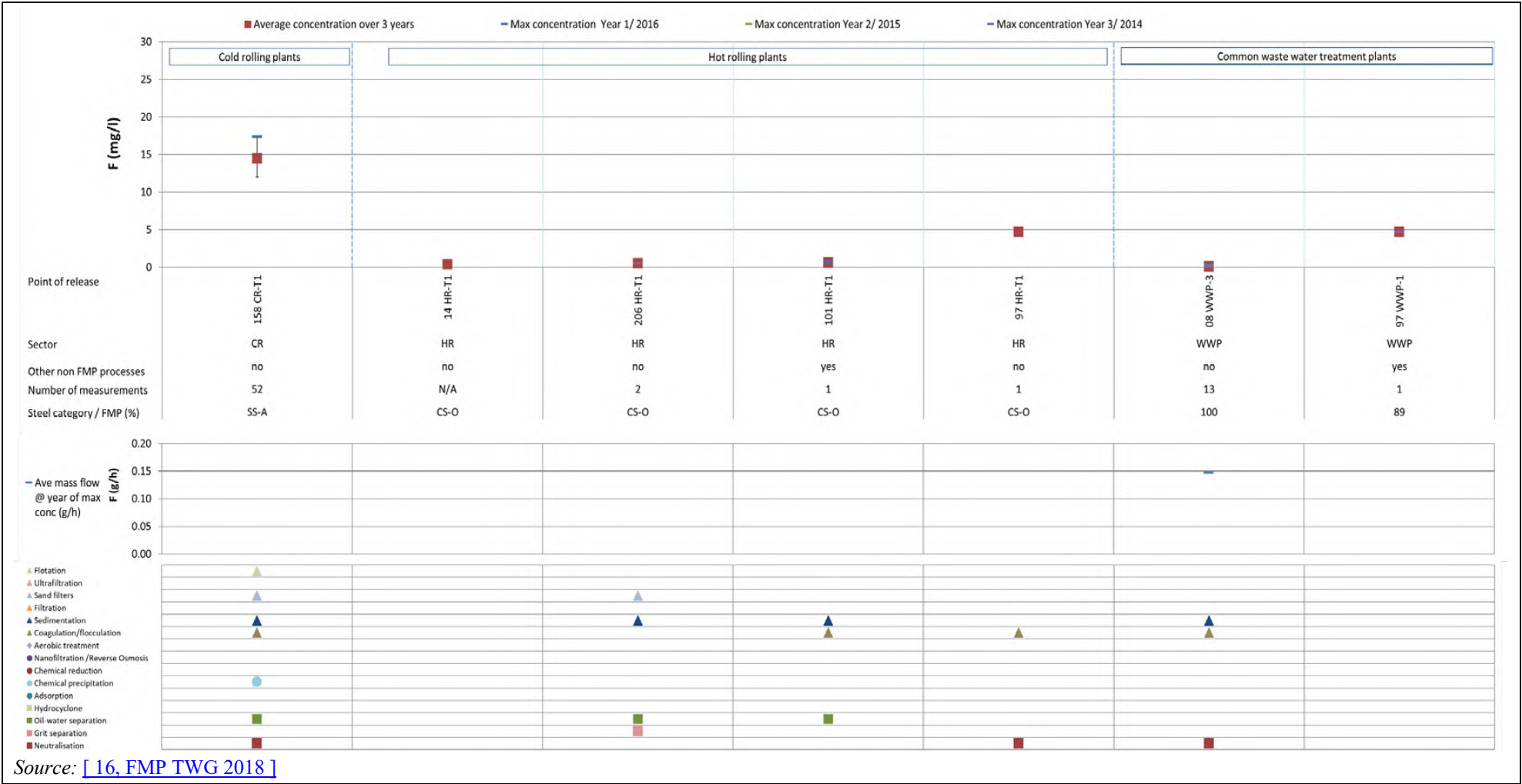
Figure 7.17: Fluoride emissions (in mg/l) for indirect discharges
