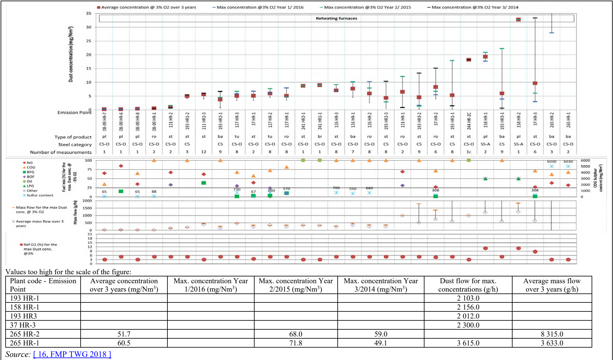
Figure 2.52: Dust emissions from feedstock heating (in mg/Nm 3 at 3 % oxygen) for fuels other than 100 % natural gas
