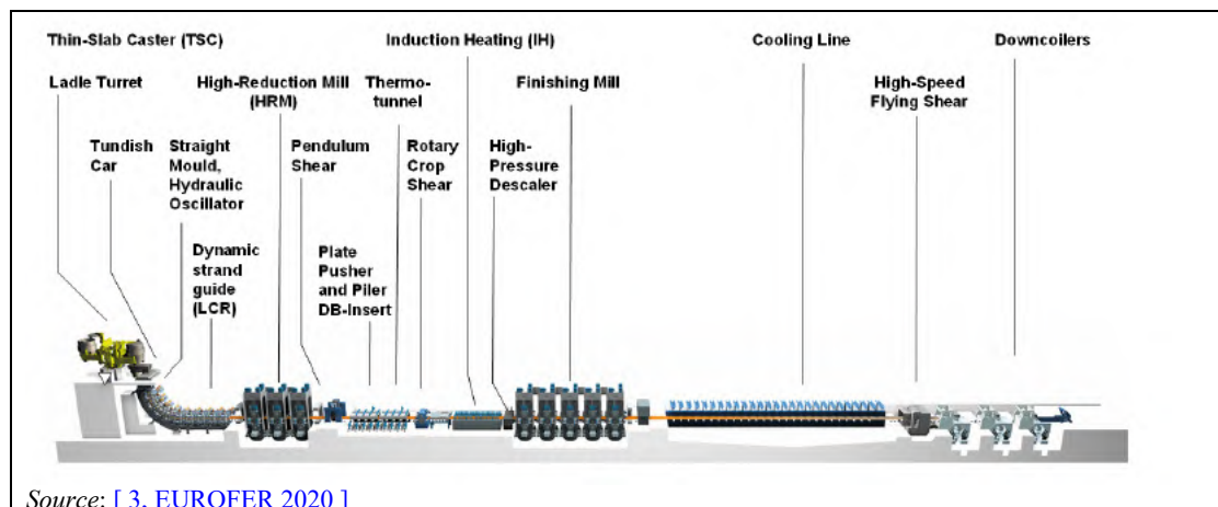
Figure 2.95: Schematic view of the Endless Strip Production process (ESP)
