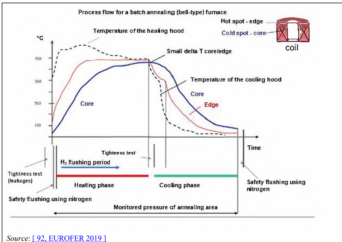
Figure 3.8: Example of temperatures during batch annealing cycle
