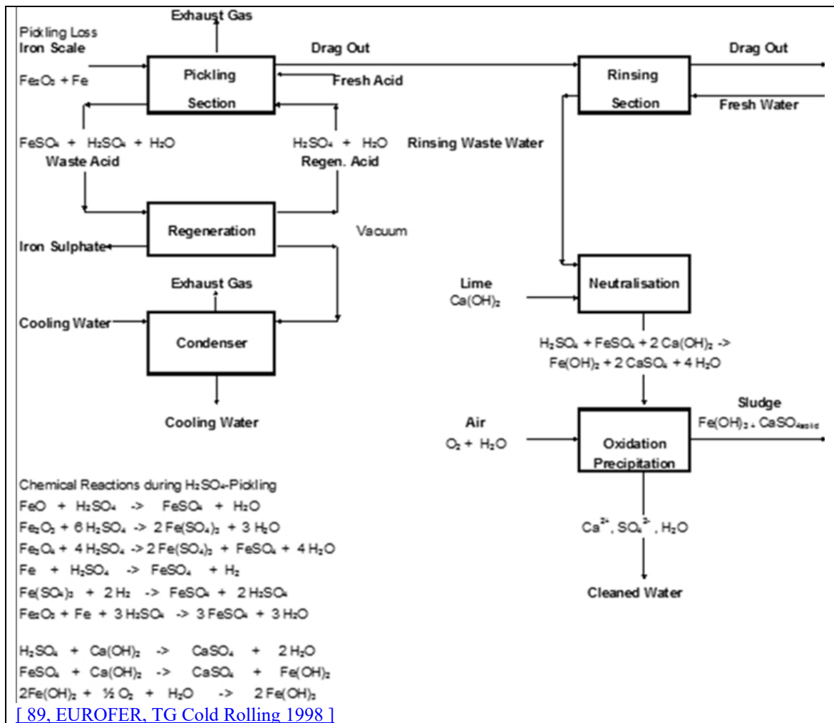
Figure 3.22: Flow sheet for H 2 SO 4 pickling and regeneration
