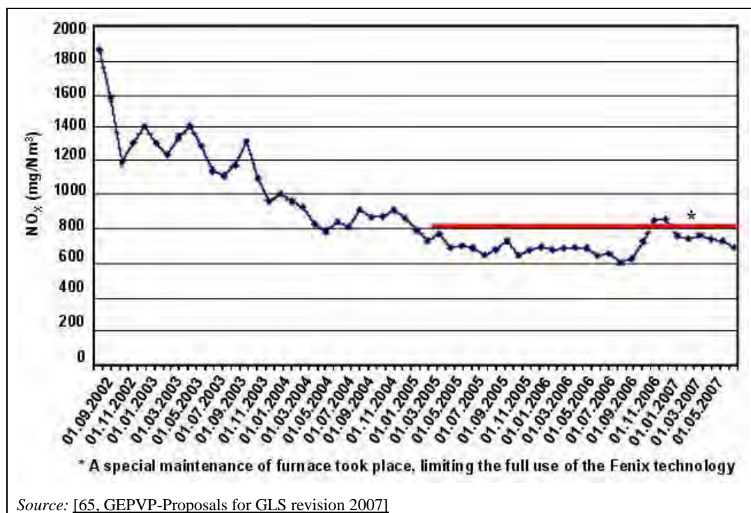
Figure 4.6: NO x emissions from the FENIX process
