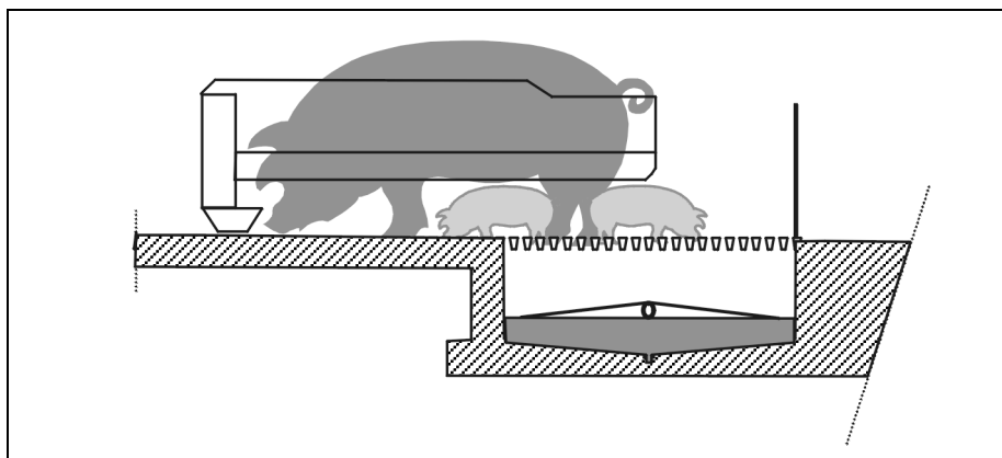
Figure 4.34: Partly-slatted floor with a manure scraper [10, Netherlands, 1999]
