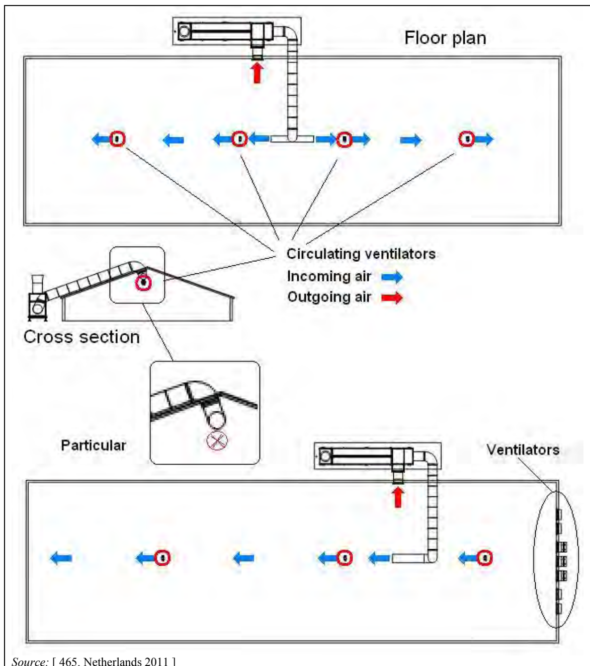
Figure 4.18: Examples of layouts for systems of circulating fans and a heat exchanger
