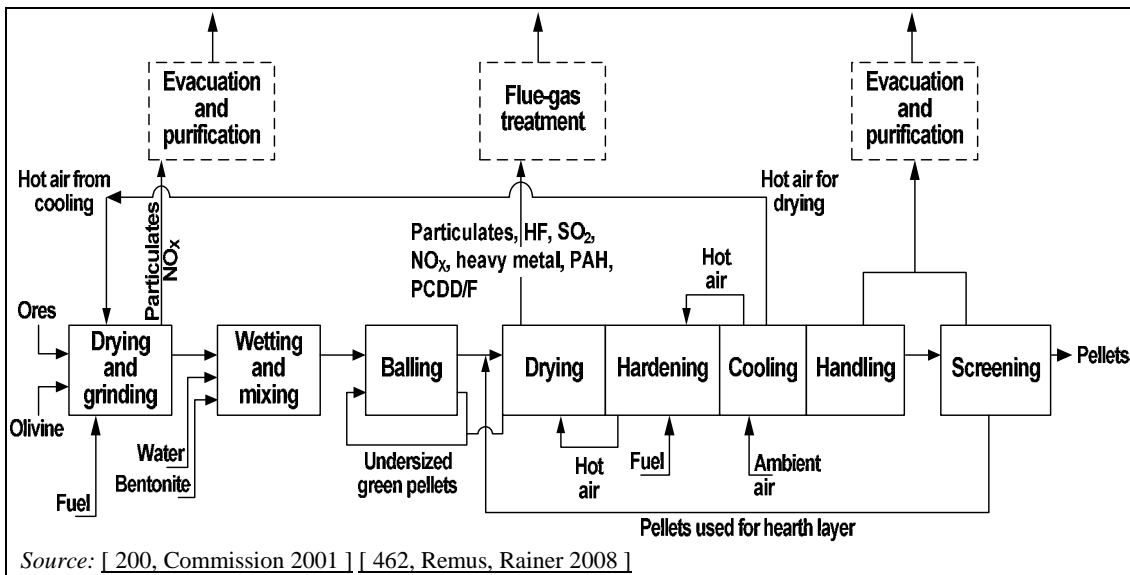
Figure 4.2: Schematic of the pelletisation plant in the Netherlands
