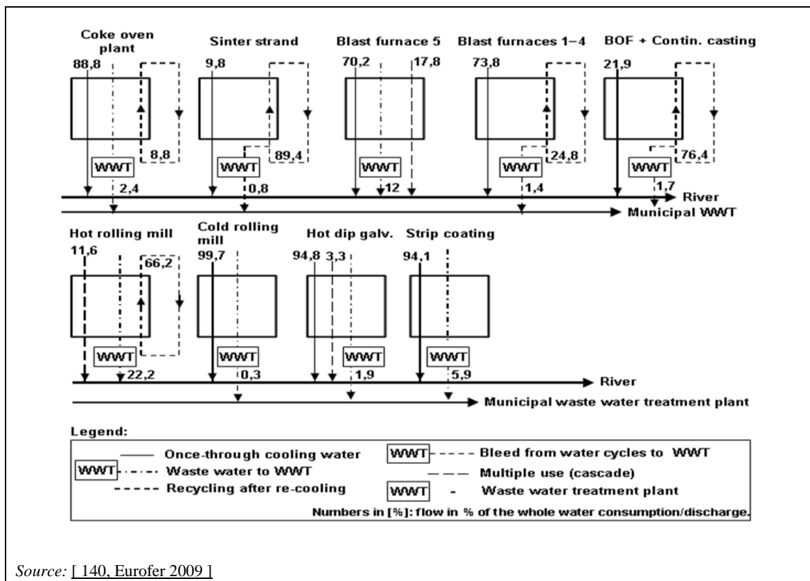
Figure 2.12: Example of water management of an integrated steelworks at a location with a high surplus of fresh water availability
