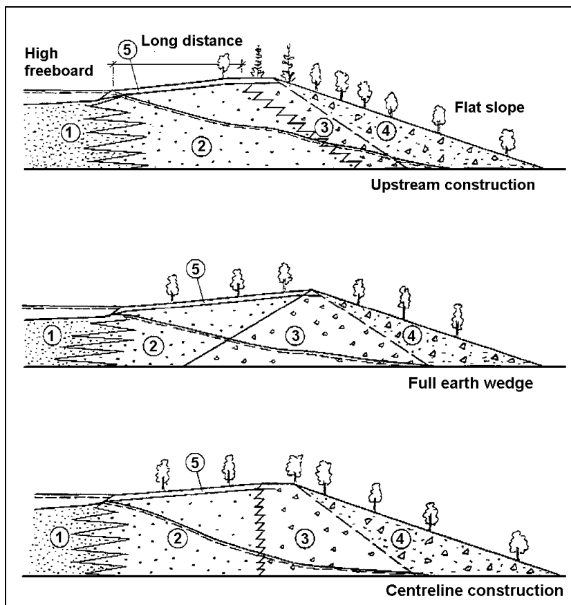
Figure 4.2: Dams for permanent water covers 1. Fine tailings, 2. Coarse tailings, 3. Support fill, 4. Support fill, long-term stable, 5. Impervious cover and erosion protection [6, ICOLD, 1996]
