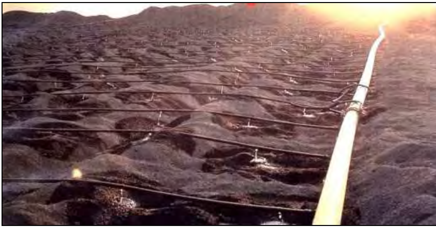
Figure 2.18: Heap leaching
