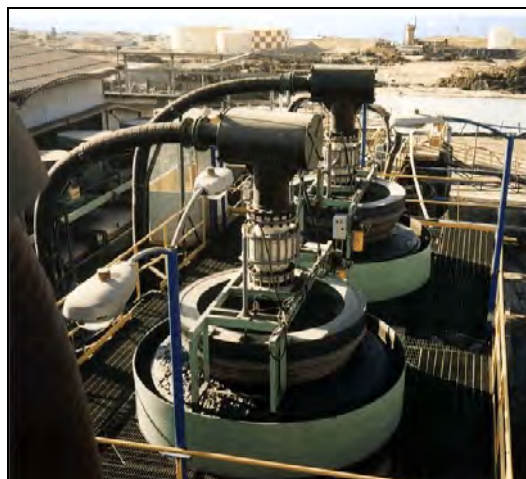
Figure 2.15: Mechanical flotation cell
