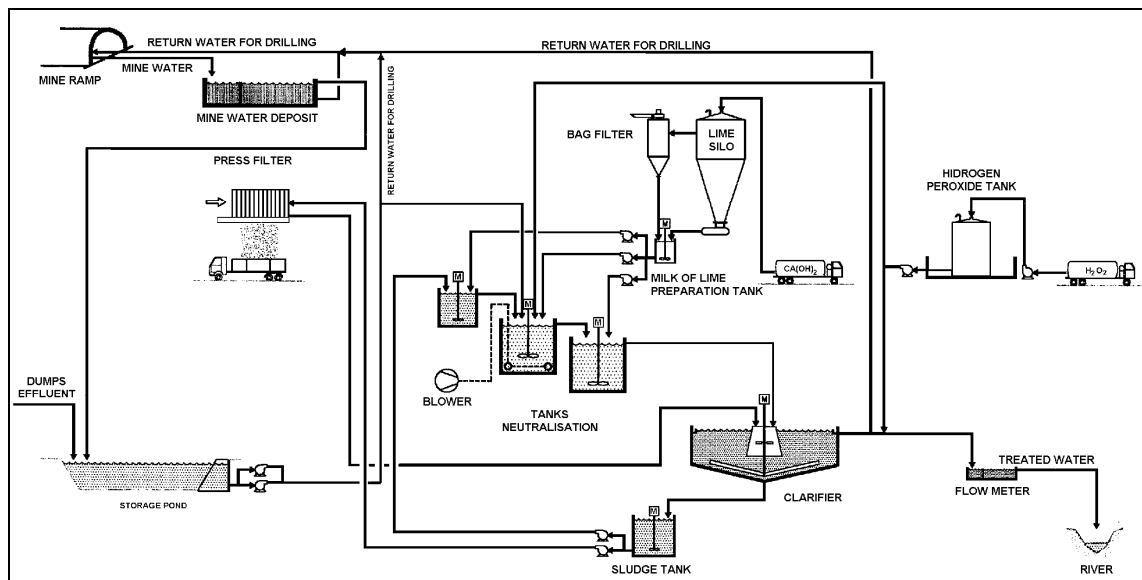
Figure 4.17: Flow sheet of a water treatment plant for low pH process water (from Almagrera)
