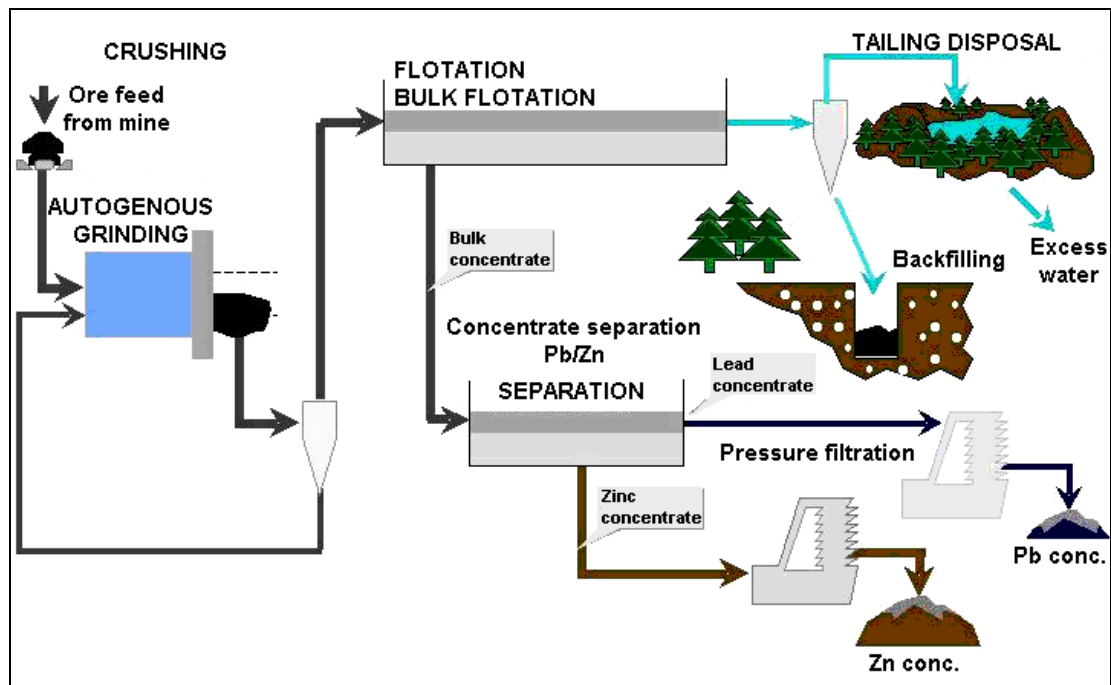
Figure 3.10: Bulk/selective flotation circuit for Zinkgruvan site [66, Base metals group, 2002]
