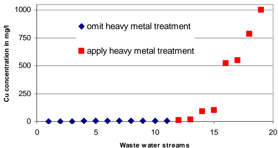
Figure 4.79: Selection of waste water streams for heavy metal treatment
