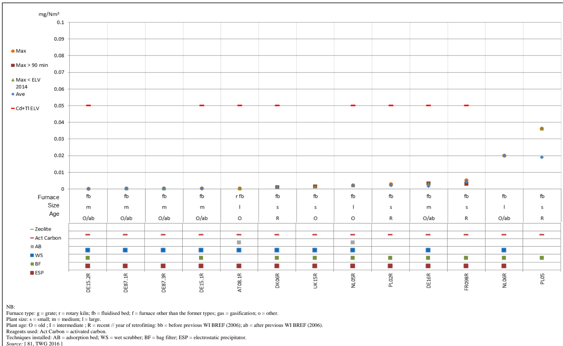
Figure 8.139: Emission levels for periodically monitored Cd+TI emissions to air from reference lines incinerating predominantly SS
