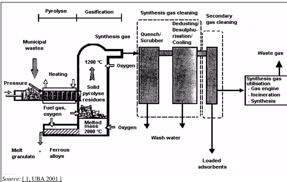
Figure 2.20: Schematic diagram of a push pyrolyser (example shown operated by Thermostelect)
