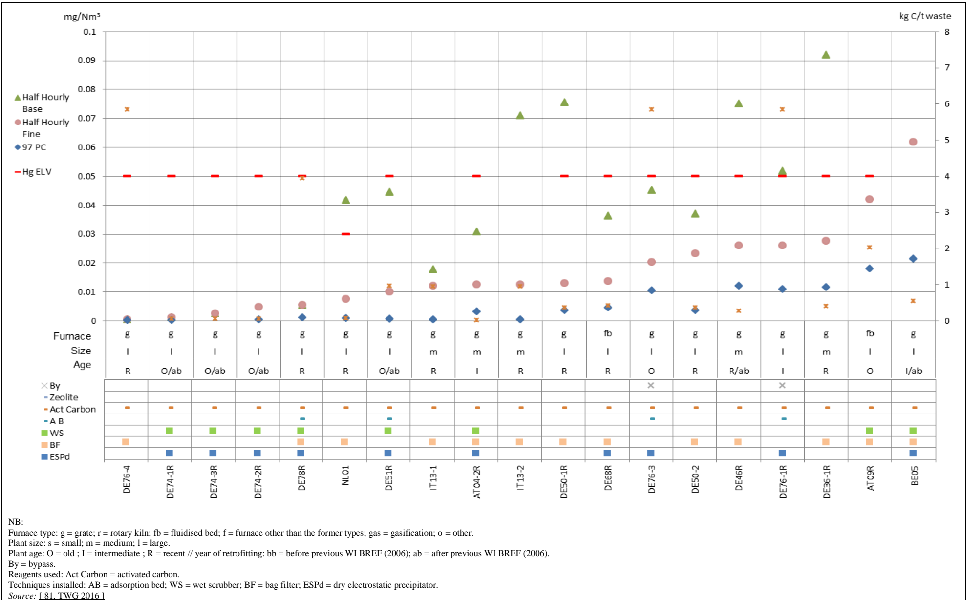
Figure 8.83: Half-hourly average emission levels for continuously monitored Hg emissions to air from reference lines incinerating predominantly ONHW
