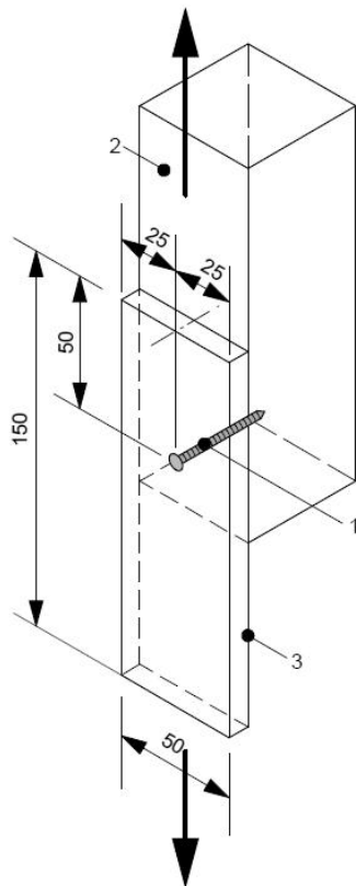
Figure 2: Principle of shear load resistance test assembly
