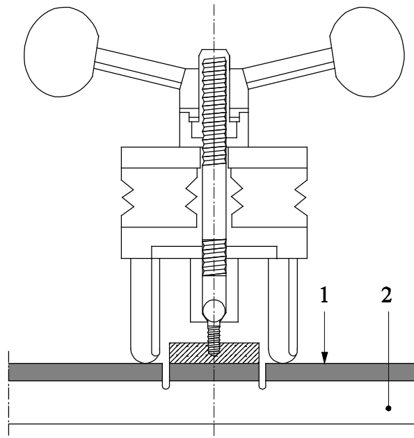
Figure 4: Principle of adhesion resistance test assembly
