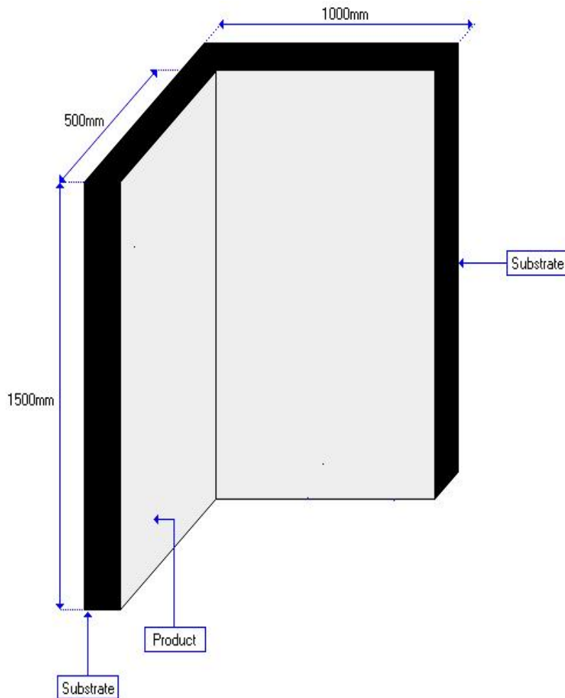
Figure A.1 – Schematic minimal jointing arrangement in EN 13823
