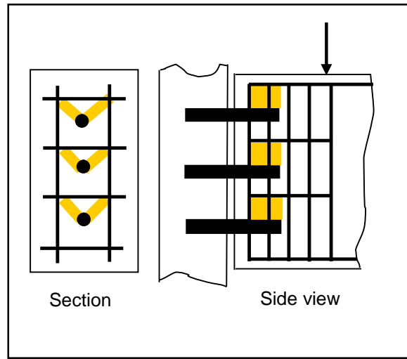
Figure A.1 – Schematic positions of reinforcements near and around superimposed dowels
