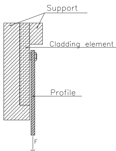
Figure 10 - Example of test of fixing
