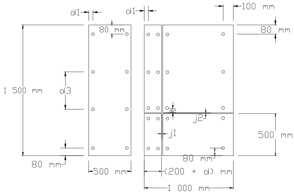
Figure E 2 - Example of installation for family A or B
