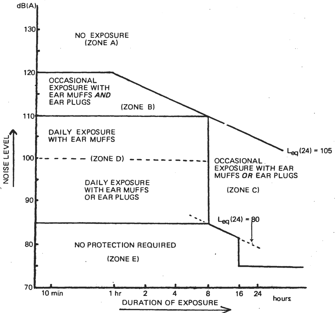
Fig. 5.1 Allowable daily and occasional noise exposure zones
