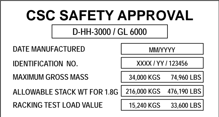
Figure 4.1 Diagram of CSC safety approval plate
